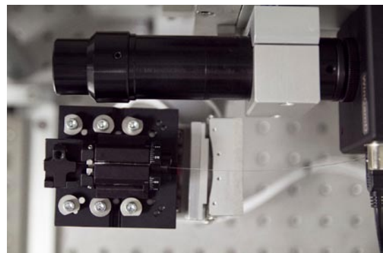
Top view of alignment stage with optical module
